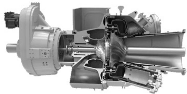
SGT-50 POWERED by SIEMENS
